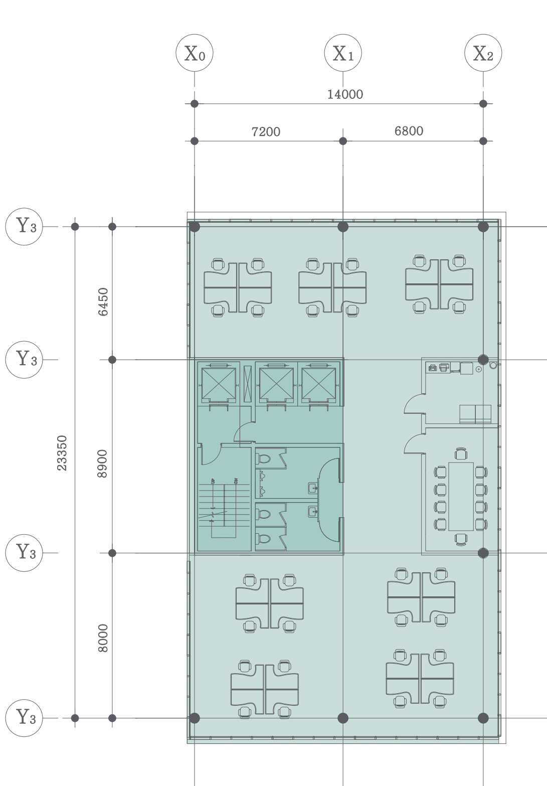
TYPICAL OFFICE PLAN SCALE 1/300
