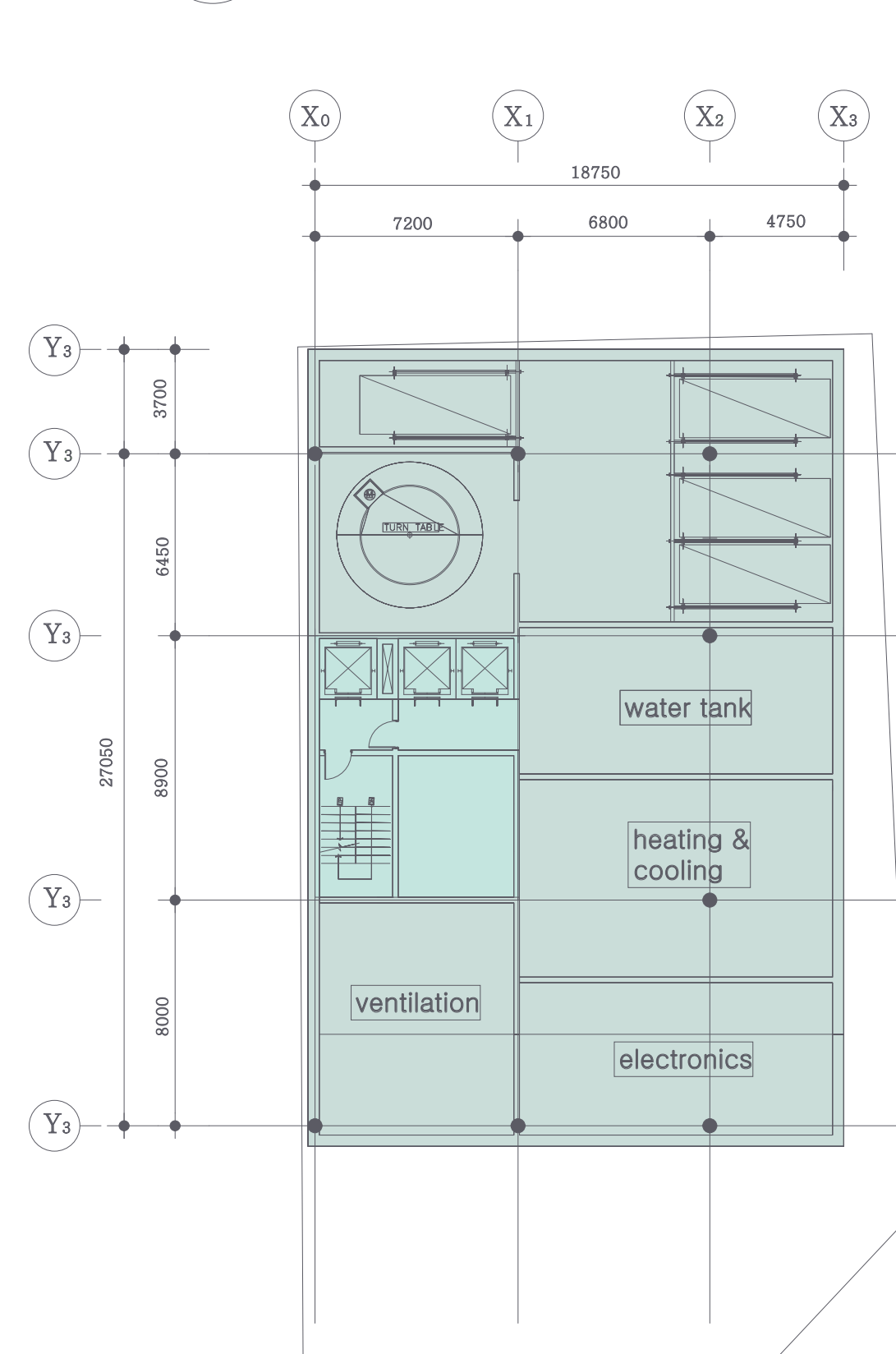
B1 FLOOR PLAN SCALE 1/300
