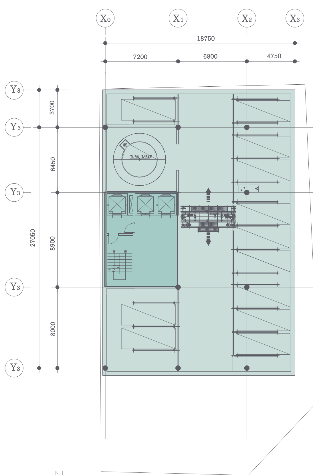
PARKING PLAN SCALE 1/300
