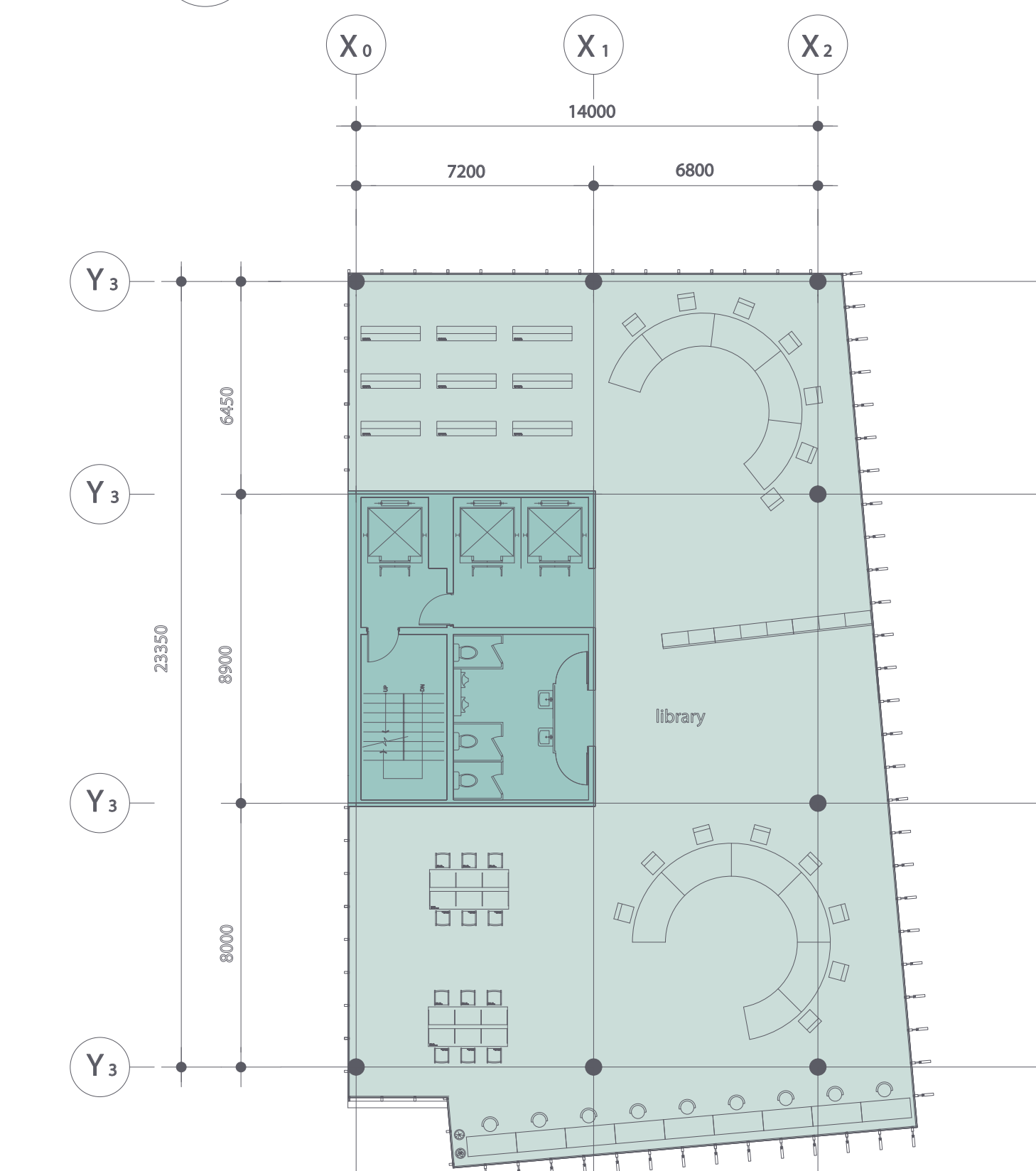
RECHARGING FLOOR PLAN SCALE 1/300
