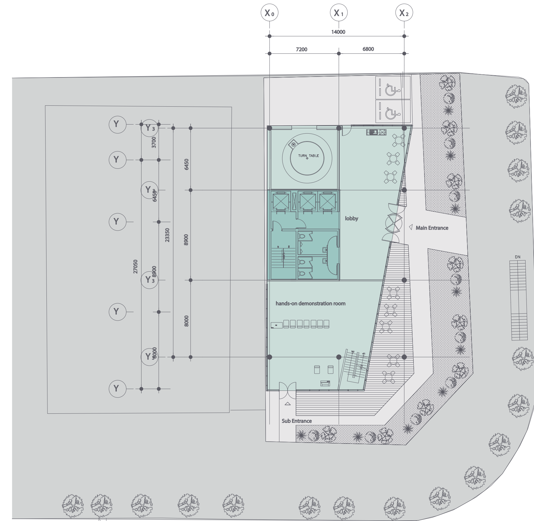
GROUND FLOOR PLAN SCALE 1/300
